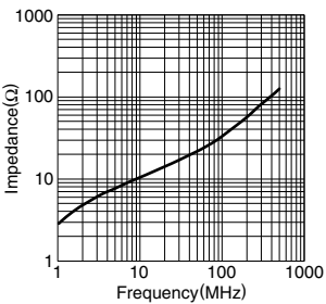
HF70SH15X0.7X8
