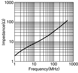
HF70SH18.8X1.1X7
