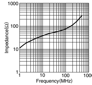
HF70SH18.8X1.1X15
