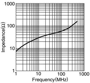
HF70SH12X0.9X12
