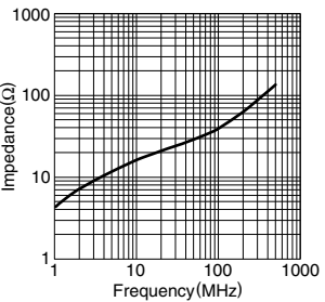
HF70SH13X0.7X10
