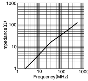
HF56SH18.8X1.1X7
