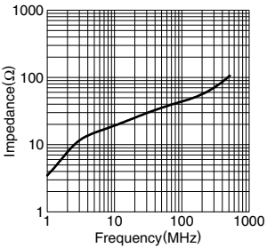
HF56SH10X1X8
