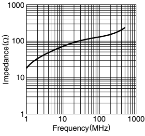
HF56SH10X1X8
